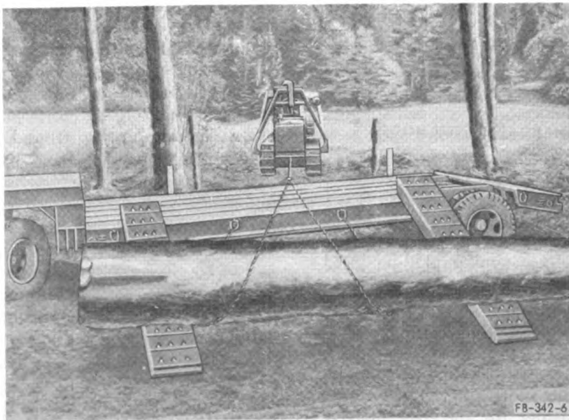
Figure 7-17. Cross-haul method of loading sawlogs.
